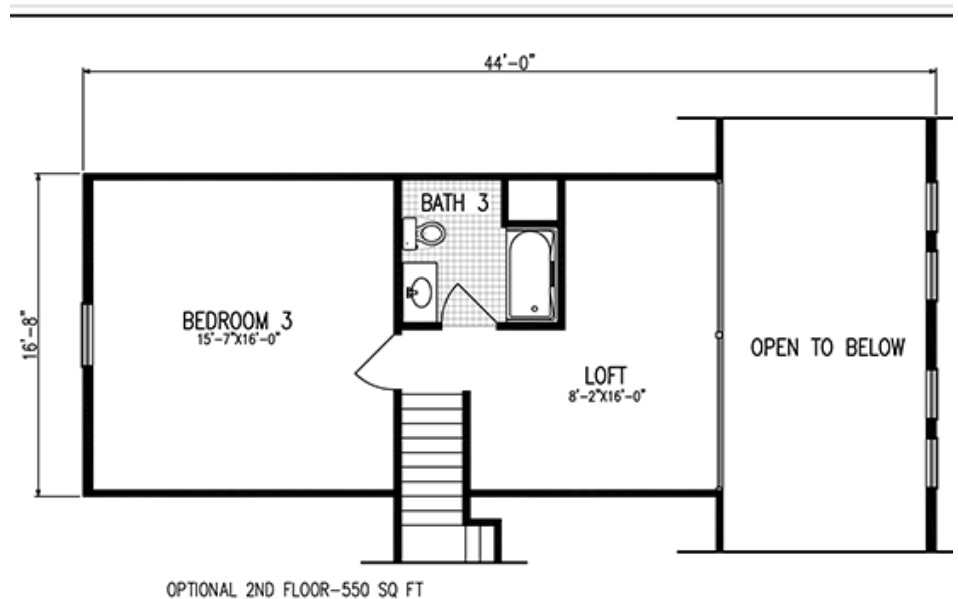
OPTIONAL 2ND FLOOR-550 SQ FT
