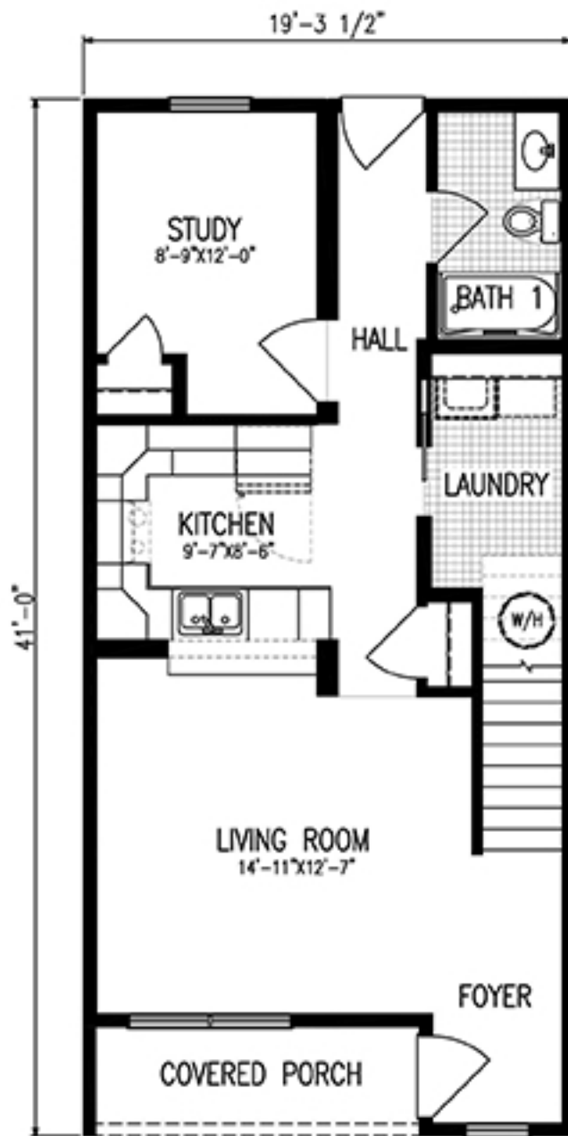
1ST FLOOR-790 SQ FT
