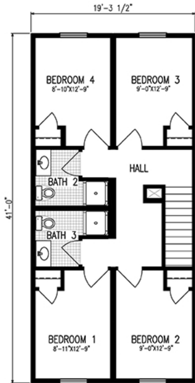
2ND FLOOR-790 SQ FT
