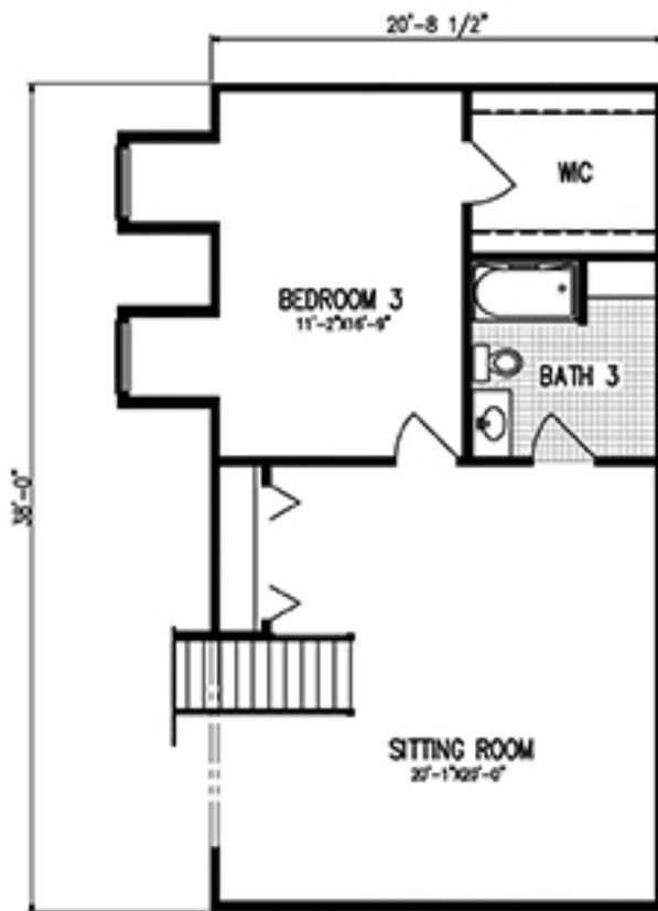
OPTIONAL 2ND FLOOR-827 SQ FT
