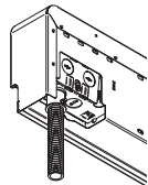
Using AC90 (BX) armoured cable from the floor (347 V to 600 V)
