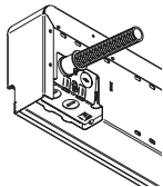
Using AC90 (BX) armoured cable from the wall (347 V to 600 V)
